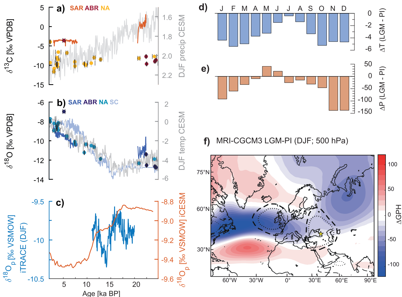
Fig. 4 Simulations and proxy records since the LGM. Carbon (a) and oxygen (b) isotope records of SAR (Sarima, highland), ABR, and NA caves (lowland). Gray lines indicate winter (DJF) precipitation (a) and winter (DJF) temperature (b) simulated by CESM transient model outputs. Dots show individual samples from NA and ABR caves (U/Th age and mean of duplicate isotope measurements) including 2- \sigma age uncertainties (black lines), whereas line plots show time series for each isotope record. The gray line in b shows the oxygen-isotope data from Sofular Cave 36 (SC). c Transient simulations of \delta^{18}\text{O} in precipitation based on iTRACE 62 and iCESM 52 at Sarima cave. MRI-CGCM3 27 monthly mean change in temperature (d) and precipitation (e) between LGM and PI simulations. f MRI-CGCM3 LGM-PI (DJF; 500 hPa) anomalies in wintertime (DJF) atmospheric structure. Color shading shows the gridded difference in DJF 500-hPa geopotential height between LGM and PI simulations. Dashed and dotted lines are the same as those in Fig. 2a, outlining the modern correlation to a mid-tropospheric dipole that influences \delta^{18}\text{O}_p at our cave sites.
