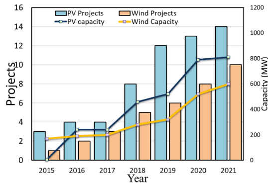
Figure 4. Jordan's renewable energy capacity growth (2015–2021) Data source: (Ministry of Energy and Mineral Resources 2022).
