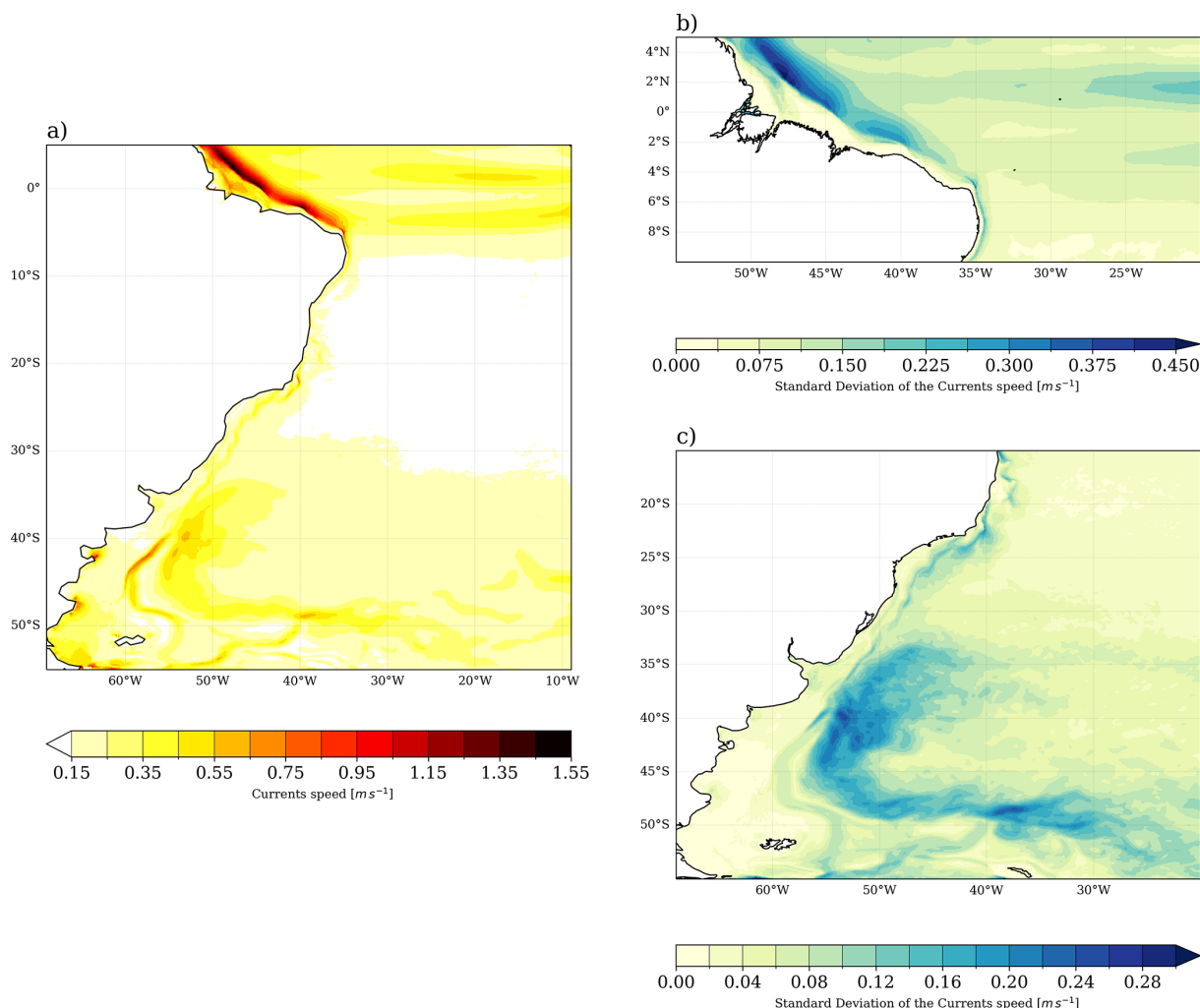
Figure 6. Mean sea surface currents ( \text{m s}^{-1} ) (a) and standard deviation of the mean speed ( \text{m s}^{-1} ) for the NBC (b) and the BMC (c) regions. The standard deviation considers the monthly variability of speed in the domain. The main BC and MC path appears with currents speed above 0.3 and 0.6 \text{ m s}^{-1} , respectively, while the speed of the NBC is above 1 \text{ m s}^{-1} .
