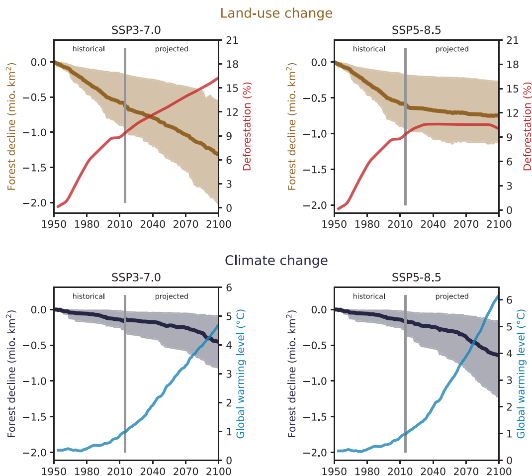
Fig. 2. Basin-wide forest decline per driver for 1950 to 2100. Annual forest decline across the Amazon basin is shown for the two drivers, land-use change and climate change, and two pathways (SSP3-7.0 and SSP5-8.5). Forest decline is shown in relation to the deforested area fraction (relative to the 1950 forest area) from the LUH2 land-use forcing and the global warming level relative to 1850 (model average), respectively. The solid lines represent the model average and the shaded areas represent the model range.
