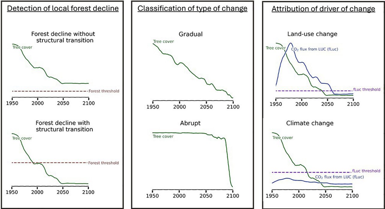
Fig. 1. Schematic overview of this study's methodology. First, we detect local (i.e., grid cell-scale) forest decline with and without a structural transition from forest to another vegetation type. A structural transition occurs when the tree cover falls below a model-specific threshold that characterizes forest vegetation (=Forest threshold). Second, we classify the forest decline as either abrupt or gradual by fitting different types of regression models that capture abrupt or gradual change to the time series of tree cover fraction. Last, we identify the driver (land-use change or climate change) of local forest decline. This is achieved by applying a model-specific threshold to the local CO 2 flux from land-use change (=fLuc), which is a proxy for the degree of local land-use change. For visualization purposes, we show the whole time period from 1950 to 2100. However, in practice, each methodological step is applied separately to the historical (1950 to 2014) and future (2015 to 2100) time series.
