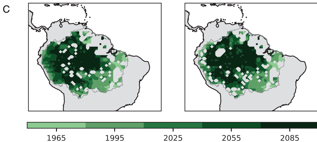
Fig. 5. Intensity and timing of forest decline across the Amazon basin. (A) Forest decline (%) relative to the 1950 forest area. Red areas in the small insets emphasize locations where forest decline includes a structural transition from forest to other vegetation. (B) Intensity of forest decline relative to the 1950 forest area per driver. Intensity (low, med(ium), high) is classified for each driver (climate change = CC or land-use change = LUC) depending on the fractional area of forest decline between 1950 and 2100: low: >0 to 20%, medium: >20 to 40%, high: >40%. Stipplings represent areas where at least three out of four models agree on the driver of forest decline. (C) Timing of the largest forest decline. The timing is classified as the year with the largest forest decline between 1950 and 2100. All values in (A–C) represent the model average for two pathways (SSP3-7.0 and SSP5-8.5). The data for each Earth System Model are regridded to a common horizontal resolution of 100 km.
