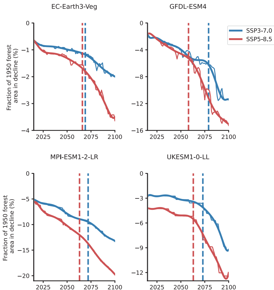
Fig. 3. Timing of nonlinear intensification of the basin-wide forest decline due to climate change across four Earth System Models for 2015 to 2100. The fraction of the 1950 forest area that is projected to decline for two pathways (SSP3-7.0 and SSP5-8.5) is shown on the y-axis. The thin lines depict the annual data, whereas the thick lines represent the (polynomial) trend. The vertical dashed lines mark the starting point of the nonlinear forest decline.
