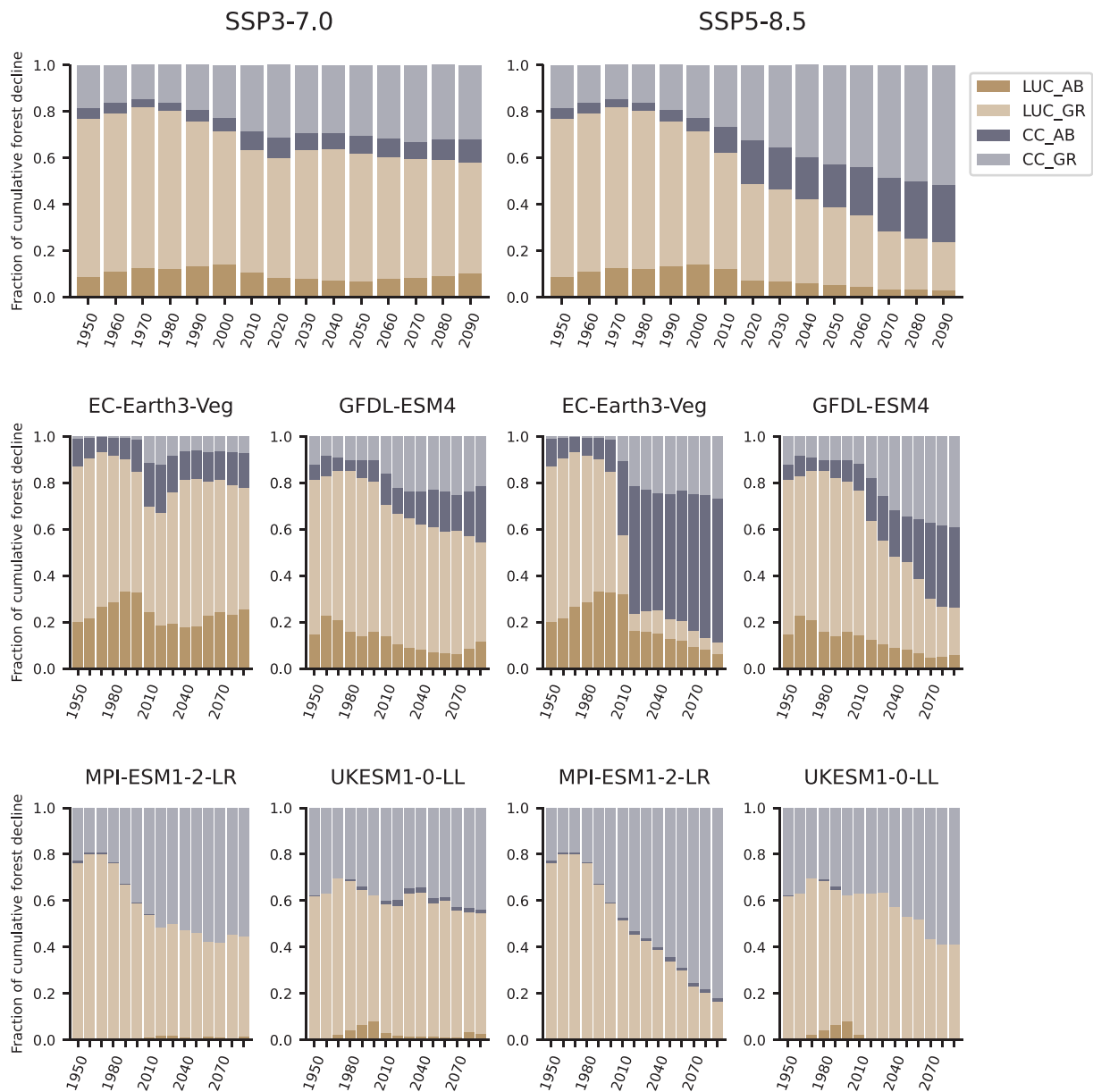
Fig. 4. Fraction of the basin-wide area of forest decline characterized by abrupt versus gradual decline for 1950 to 2100. The numbers indicate the 10-y average fraction of the regional area of forest decline (relative to 1950) caused by each driver (CC = climate change or LUC = land-use change) and characterized by either abrupt (=AB) or gradual (=GR) decline for two pathways (SSP3-7.0 and SSP5-8.5). The average across four models is shown in the first row and the individual Earth System Models are shown in the second and third rows.
