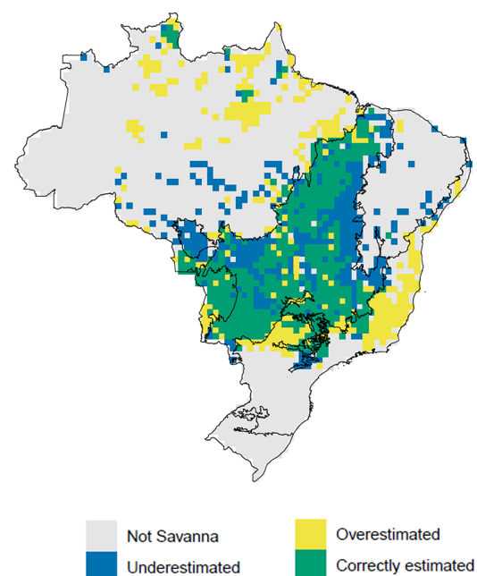
Figure 4. Maps showing the Brazilian vegetation types according to IBGE (left) and TrBS PFT distribution accuracy (right) in comparison with the savanna vegetation class from IBGE. A threshold of 30 % FPC cover was used to determine distribution accuracy.
