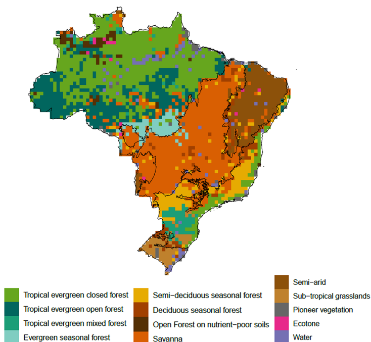
Figure 4. Maps showing the Brazilian vegetation types according to IBGE (left) and TrBS PFT distribution accuracy (right) in comparison with the savanna vegetation class from IBGE. A threshold of 30 % FPC cover was used to determine distribution accuracy.
