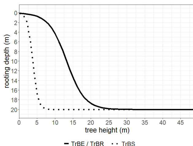
Figure 2. Logistic growth function scaling rooting depth to tree height, shown for a soil depth of 20 m for the different PFTs (TrBE: tropical broadleaved evergreen, TrBR: tropical broadleaved rain-green, TrBS: Tropical Broadleaved Savanna).
