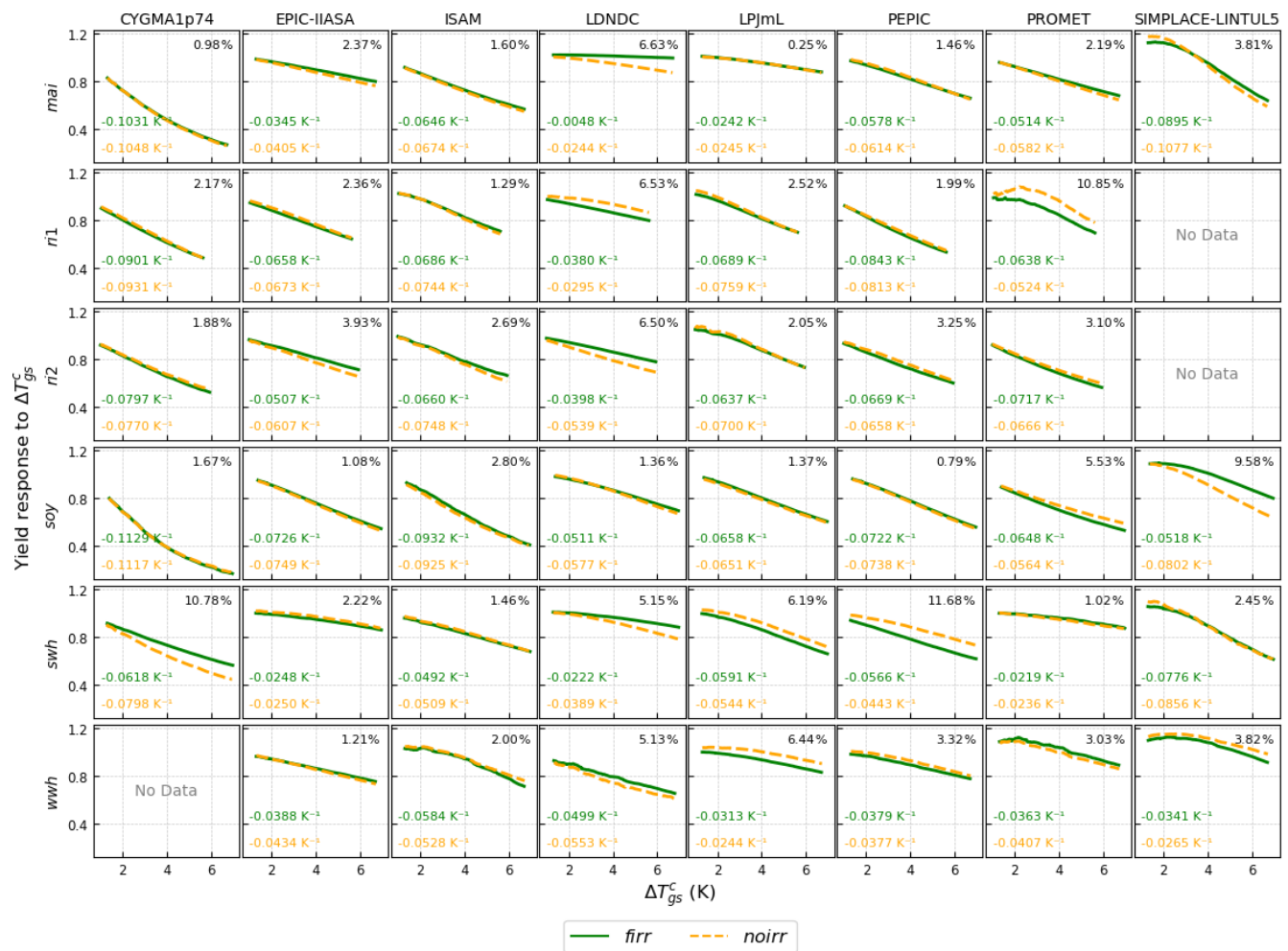
Figure 4. Global crop yield responses to growing season temperature change (K) across eight GGCMs (extreme-value regions masked), showing firr (green solid lines) and noirr (orange dashed lines) crop yield response sensitivity to growing season temperature change under SSP585, and RRMSE (%) between firr and noirr crops across GGCM-crop combinations. Sensitivity values for firr and noirr crops are shown in green and orange, respectively, with their RRMSE values reported in the upper-right corner.
