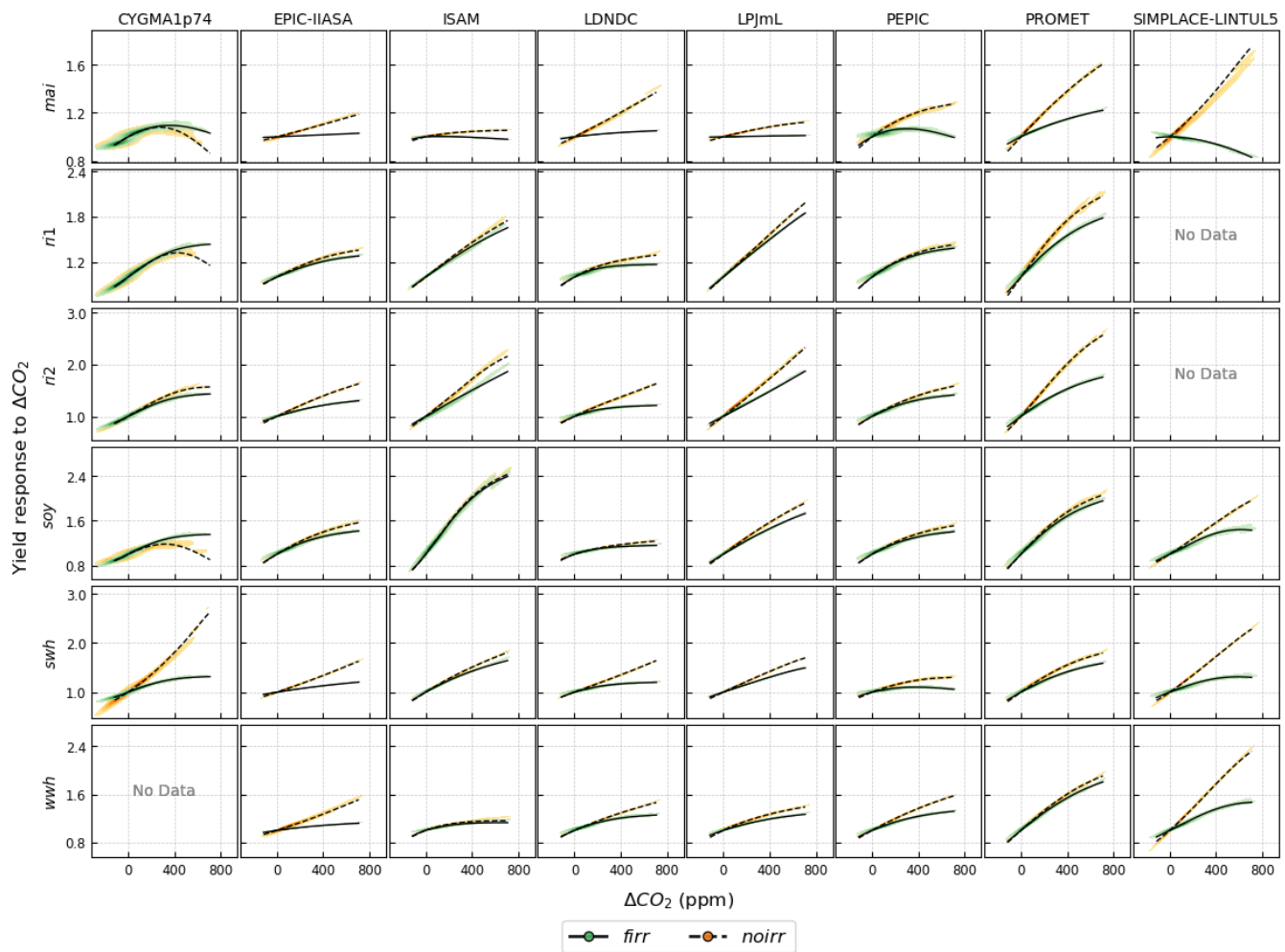
Figure 3. Kernel density estimation of global crop yield responses to [\text{CO}_2] change (ppm) across eight GGCs under historical, SSP126, SSP370, and SSP585, with extreme-value regions masked. Black lines indicate aggregated results from the crop emulator. Green shades and orange shades represent firr and noirr conditions, separately. Darker shades suggest higher density.
