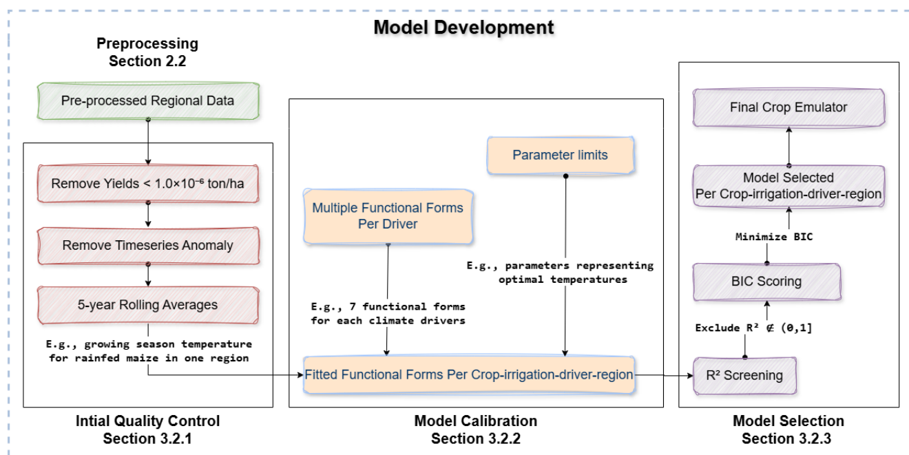
Figure 2. Flowchart of model development procedure.
