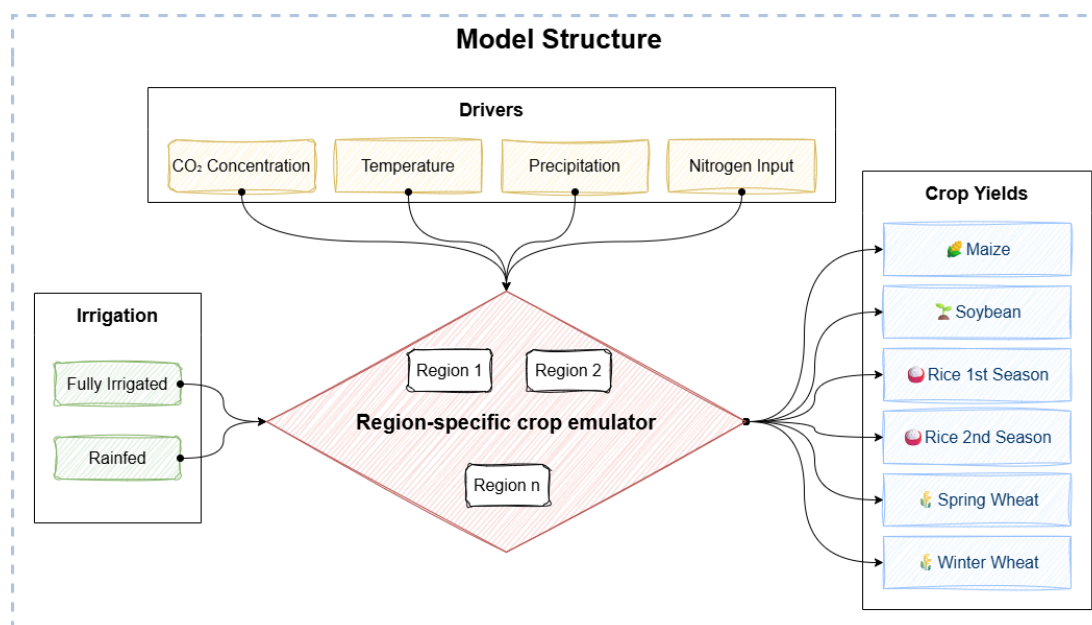
Figure 1. Crop yield emulator structure.
