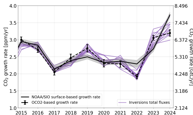
Figure 9. Annual atmospheric CO 2 growth rates based on observations from the surface network (by NOAA (National Oceanic and Atmospheric Administration) and SIO (Scripps Institution of Oceanography)), as well as using the Growth Rate from Satellite Observations (GRESO) approach using OCO-2 based XCO 2 observations in ppm yr −1 with uncertainties. To obtain G_{\text{ATM}} , the surface observation-based growth rate in units of ppm yr −1 is converted to units of GtC yr −1 by multiplying by a conversion factor (CF) of 2.124 GtC ppm −1 , assuming instantaneous mixing of CO 2 throughout the atmosphere. The purple lines are the atmospheric growth rates (in GtC yr −1 ) calculated as the sum of the fluxes derived by the atmospheric inversions. Note that the right hand axis shows the growth rate in GtC yr −1 , with intervals of the conversion factor.
