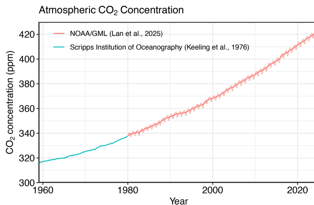
Figure 1. Surface average atmospheric CO 2 concentration (ppm). Since 1980, monthly data are from NOAA/GML (Lan et al., 2025) and are based on an average of direct atmospheric CO 2 measurements from multiple stations in the marine boundary layer (Masarie and Tans, 1995). The 1958–1979 monthly data are from the Scripps Institution of Oceanography, based on an average of direct atmospheric CO 2 measurements from the Mauna Loa and South Pole stations (Keeling et al., 1976). To account for the difference of mean CO 2 and seasonality between the NOAA/GML and the Scripps station networks used here, the Scripps surface average (from two stations) was de-seasonalised and adjusted to match the NOAA/GML surface average (from multiple stations) by adding the mean difference of 0.667 ppm, calculated here from overlapping data during 1980–2012.
