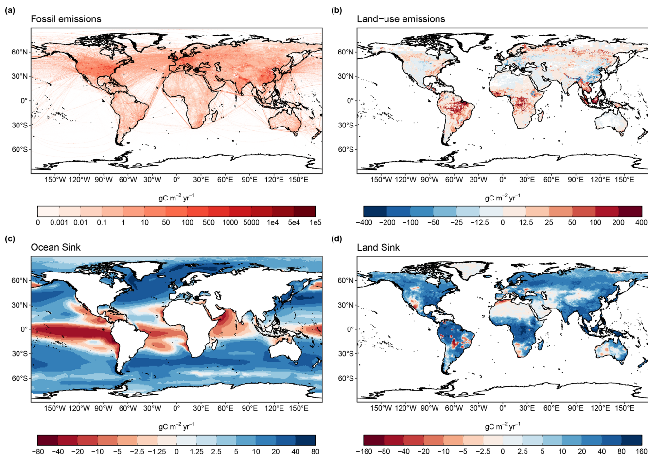
Figure 6. The 2015–2024 decadal mean components of the global carbon budget, presented for (a) fossil CO 2 emissions ( E_{\text{FOS}} ), (b) land-use change emissions ( E_{\text{LUC}} ), (c) the ocean CO 2 sink ( S_{\text{OCEAN}} ), and (d) the land CO 2 sink ( S_{\text{LAND}} ). Positive values for E_{\text{FOS}} and E_{\text{LUC}} represent a flux to the atmosphere, whereas positive values of S_{\text{OCEAN}} and S_{\text{LAND}} represent a flux from the atmosphere to the ocean or the land (carbon sink). In all panels, red colours represent a source (flux from the land/ocean to the atmosphere), blue colours represent a sink (flux from the atmosphere into the land/ocean). All units are in \text{gC m}^{-2} \text{yr}^{-1} . Note the different scales in each panel. E_{\text{FOS}} data shown is from GCP-GridFEDv2025.0 and does not include cement carbonation. The E_{\text{LUC}} map shows the average E_{\text{LUC}} from the three bookkeeping models plus emissions from peat drainage and peat fires. BLUE and LUCE provide spatially explicit estimates at 0.25^\circ resolution. Gridded E_{\text{LUC}} estimates for OSCAR are derived by spatially distributing their national data based on the spatial patterns of BLUE gross fluxes in each country (see Schwingshackl et al. (2022), for more details about the methodology). S_{\text{OCEAN}} data shown is the average of un-adjusted GOBMs and f\text{CO}_2 -products means, using GOBMs simulation A, no adjustment for bias and drift applied to the gridded fields (see Sect. 2.5). S_{\text{LAND}} data shown is the average of the DGVMs for simulation S2, no adjustment for bias and drift applied to the gridded fields (see Sect. 2.6).
