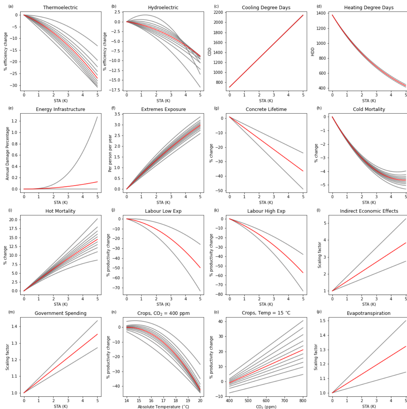
Figure A1. Panel plot of the climate impact channel functions displayed in Fig. 1 and described in Sect. 2.1–2.6. Red curves represent the median central estimate, with grey giving the uncertainty variation. In cases in which uncertainty is treated by “Sampled Percentiles” in Table 1, the 11 parameter sets representing the 2.5th to 97.5th percentiles, with equal spacing, are shown; for the other impact channels, the range using the upper and lower parameter values after literature analysis and internal calibration is shown.
