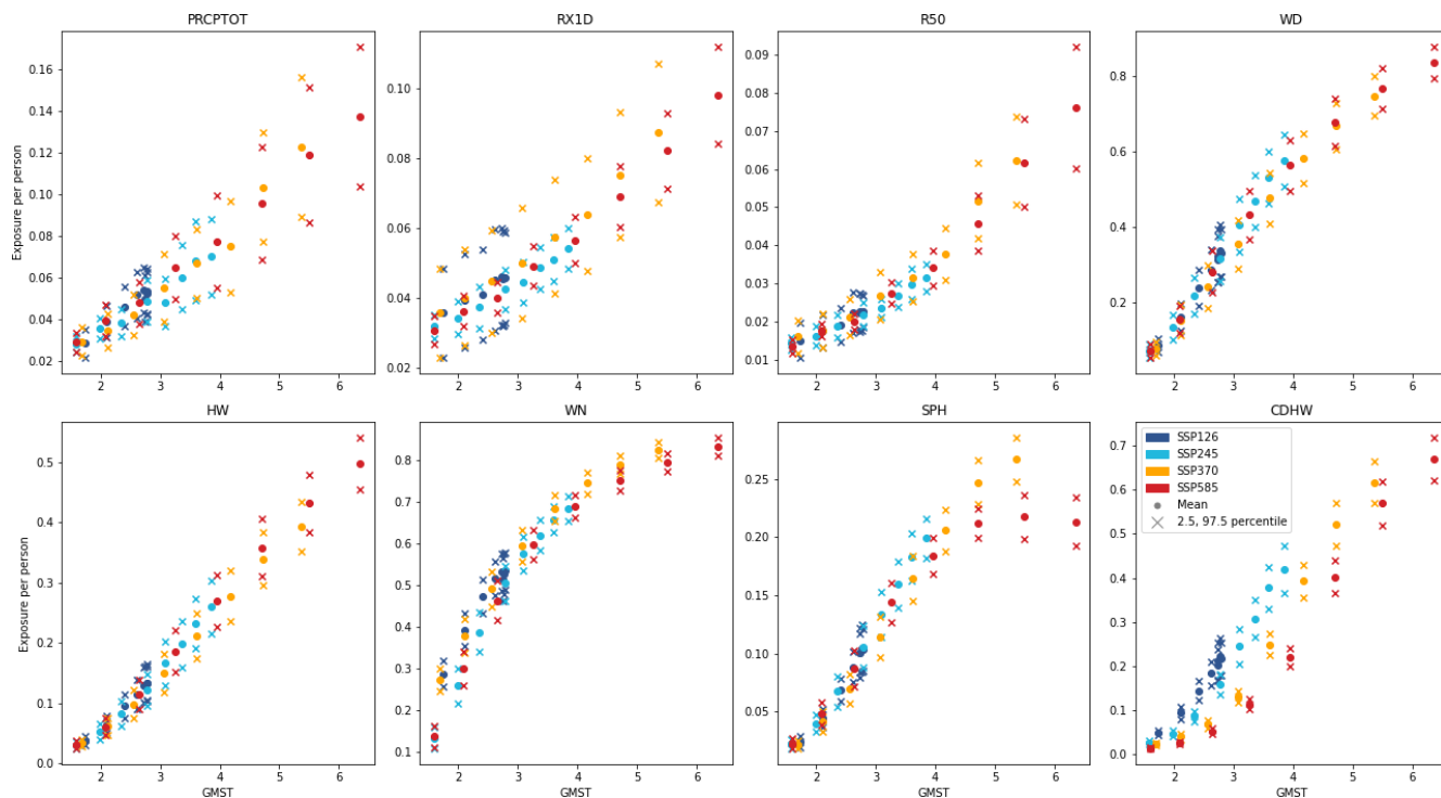
Figure A4. Changes in population-weighted exposure to extremes of various climate metrics, under multiple scenarios, as a function of global mean temperature. The mean and 2.5th and 97.5th percentile values across 21 climate models are shown.
