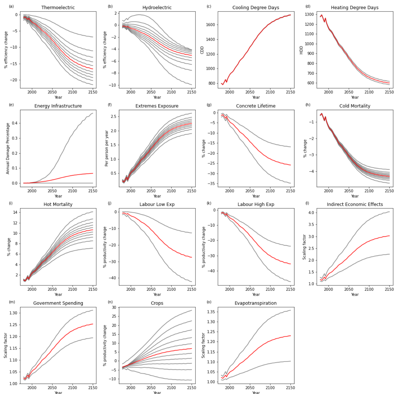
Figure A2. Panel plot of the timeseries response of the impact functions under a baseline scenario in FRIDA which reaches 3.5 K temperature change and 730 ppm CO 2 concentrations by 2150 (see Code and Data Availability). Parameter sets shown as in Fig. A1; note that the crop response combines the temperature and CO 2 effects here.
