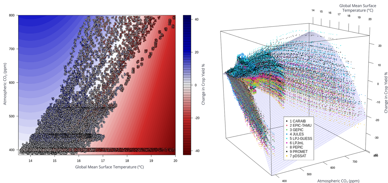
Figure A5. Response in crop yield as a function of global mean temperature and CO 2 concentrations. Individual data points represent climate model-crop model combinations from Müller et al. (2021), annually resolved. Data from multiple future SSP scenarios as well as idealised fixed-CO 2 versions are shown. Left panel shows the CO 2 – GMST combinations, with the chosen fit shown in coloured contours, and the annual model data as coloured datapoints. Right panel shows the results in 3D space, with the yield response in the 3rd dimension.
