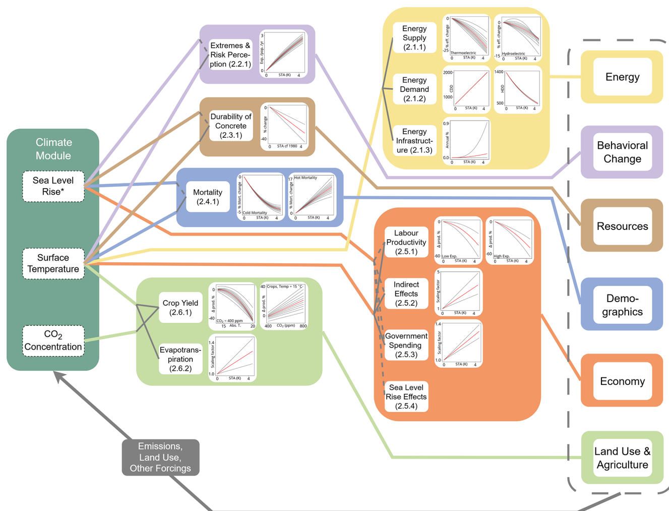
Figure 1. Outputs from the Climate module (left), and their linkages to other modules in FRIDAv2.1 (right) via climate impact channels. Coloured lines and groupings indicate the module affected by each set of impacts; grey lines inside the central boxes show the specific drivers of each damage. Each numbered box represents a distinct climate impact channel, with its implementation process described in the corresponding part of Sect. 2. Graphs to the right of each channel name show the damage function(s) implemented as part of that impact channel; see Fig. A1 for a more detailed version of these graphs. Within the graphs, red curves represent the median central estimate, with grey giving the uncertainty variation. In cases in which uncertainty is treated by “Sampled Percentiles” in Table 1, the 11 parameter sets representing the 2.5th to 97.5th percentiles, with equal uncertainty spacing, are shown; for the other impact channels, the range using the upper and lower parameter values after literature analysis and internal calibration is shown. Completion of the human–Earth system feedback loops, via the cascading effect on human drivers of the Earth system response, is represented schematically by the grey arrow. * Sea Level Rise impacts are indicated in this figure, but generally cannot be reduced to a single function, and therefore are not represented in the plots. Instead these are discussed in their respective sections and Ramme et al. (2025).
