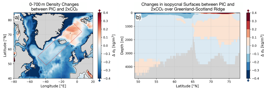
Figure 5. Density changes under elevated atmospheric \text{CO}_2 concentration averaged over 20 model years. Panel (a) is depicting density changes in the upper 700 m between the CM2.6 PIC run and the 2 \times \text{CO}_2 scenario. Panel (b) is showing the latitude-depth cross section of the red box in (a).
