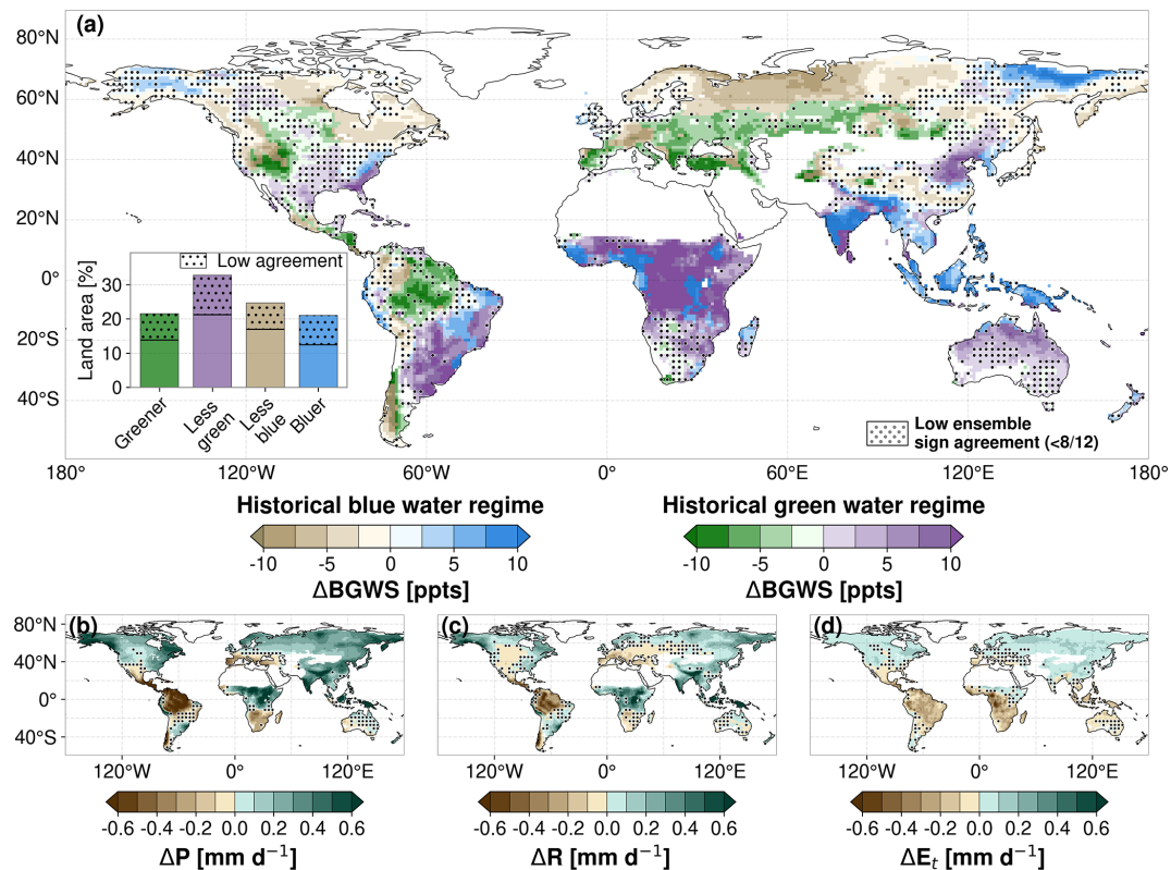
Figure 2. Ensemble mean change (2071–2100 minus 1985–2014) under the SSP3-7.0 scenario based on 12 CMIP6 Earth system models. (a) \Delta\text{BGWS} [ppts], shown separately for grid cells with historically positive BGWS values (blue water regime; beige to blue colours) and historically negative BGWS values (green water regime; green to purple colours). Blue and purple colours indicate shifts towards larger blue water shares, whereas green and beige colours indicate shifts towards larger green water shares. The inset summarises the analysed land-area fractions of the four BGWS-change classes; bar heights show the total area of each class, the horizontal line marks the fraction with robust sign agreement, and the stippled upper part indicates the fraction with low model agreement. (b) \Delta precipitation [ \text{mm d}^{-1} ], (c) \Delta runoff [ \text{mm d}^{-1} ], and (d) \Delta transpiration [ \text{mm d}^{-1} ]. All panels use the fixed historical analysis mask described in Sect. 2.3. Stippling marks regions of low inter-model agreement, where fewer than 8 of the 12 models agree on the sign of change.
