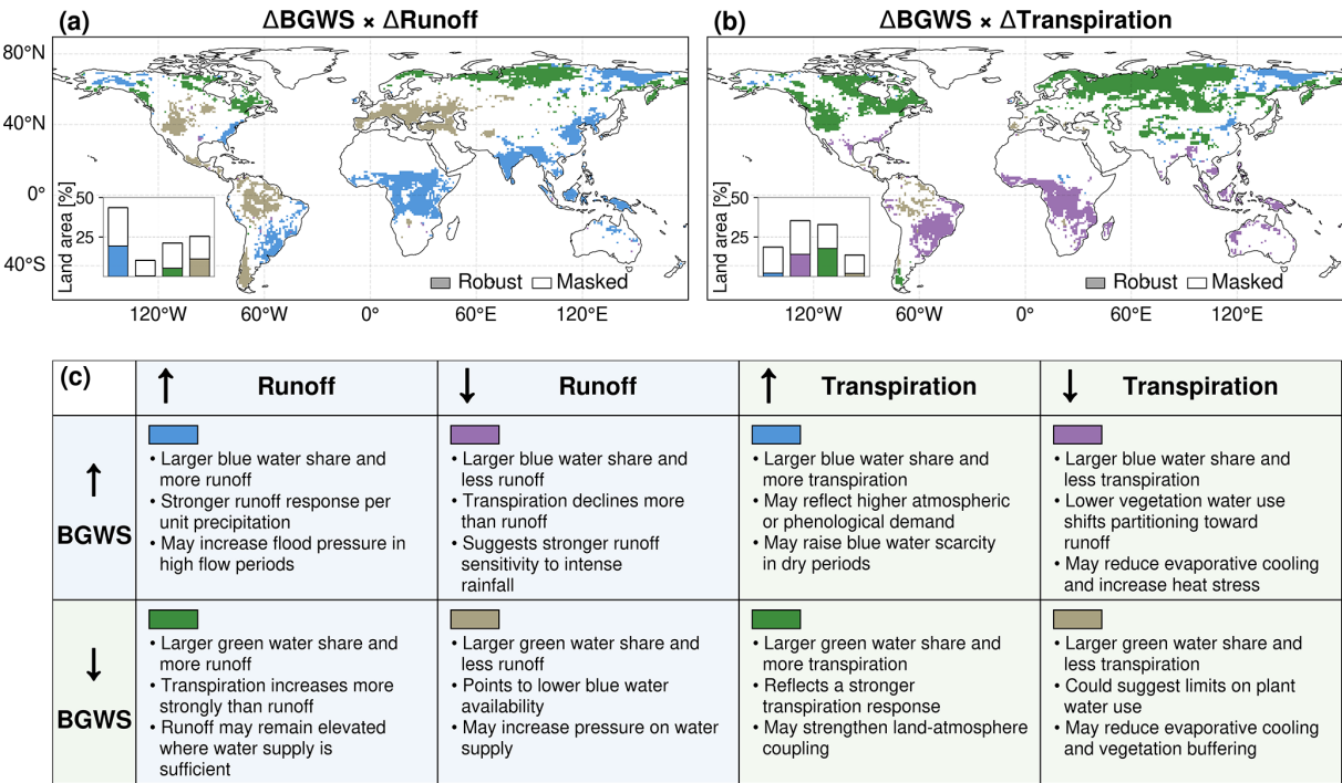
Figure 4. Projected changes in blue–green water partitioning and associated runoff and transpiration responses. Panels (a) and (b) show the ensemble mean \Delta\text{BGWS} combined with changes in runoff and transpiration, respectively, for the end of the century relative to the historical period. Colours indicate the four joint sign combinations between \Delta\text{BGWS} and the corresponding flux change, as defined schematically in panel (c), which also summarises their possible hydroecological implications. White grid cells in panels (a) and (b) denote areas excluded by the fixed historical analysis mask (Sect. 2.3) or masked because fewer than 8 of the 12 models agree on the same joint quadrant class. Insets show the land-area fraction of each quadrant class, with coloured bar segments indicating robust area and white segments indicating area masked because of low agreement.
