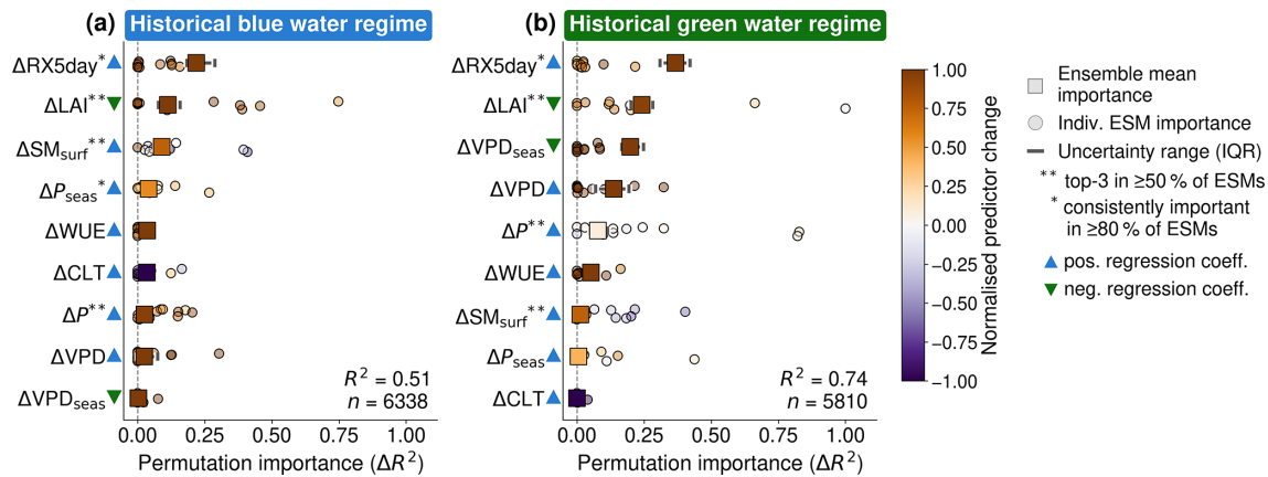
Figure 3. Variable importance for the spatial attribution of projected changes (2071–2100 minus 1985–2014) in \Delta\text{BGWS} under the SSP3-7.0 scenario in the two historical BGWS regimes shown in Fig. 2: (a) historical blue water regime and (b) historical green water regime. Squares show the median permutation importance ( \Delta R^2 ) of the 12-model CMIP6 ensemble mean for the predictor set, and horizontal lines show the interquartile range across repeated blocked cross-validation splits. Circles show the median permutation importance from individual ESMs with mean model performance R^2 > 0.3 . Colours indicate the normalised mean change of each predictor within the respective regime. Upward blue triangles indicate positive regression coefficients and downward green triangles indicate negative regression coefficients in the ensemble mean. Reported R^2 values give the mean model performance. The attribution is fitted only for grid cells retained by the fixed historical analysis mask described in Sect. 2.3; n gives the number of retained grid cells in each regime.
