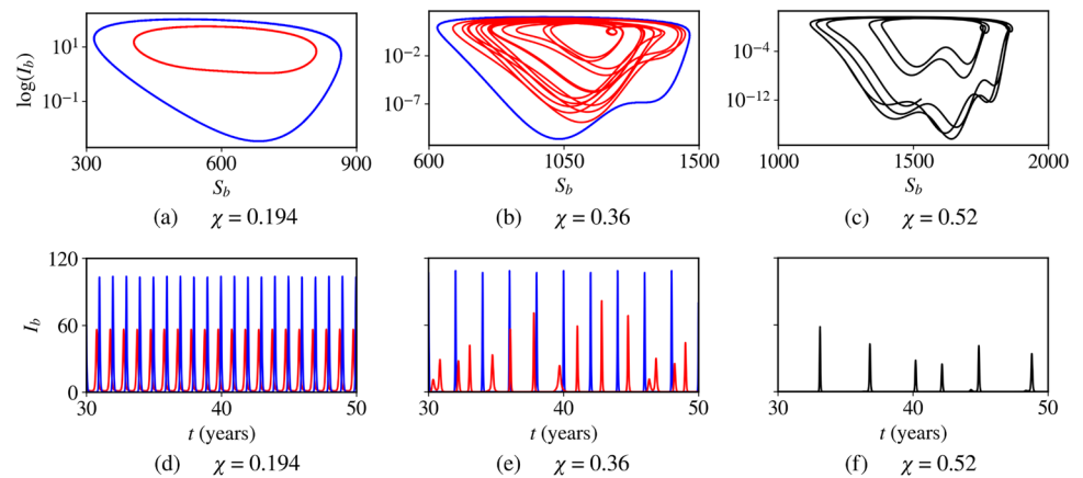
Fig. 4 Projections of the attractors onto the S_b \times I_b plane for \chi = 0.194 , 0.36 , and 0.52 in panels a–c , respectively. The corresponding time series of I_b associated with each attractor are shown in panels d–f , respectively
