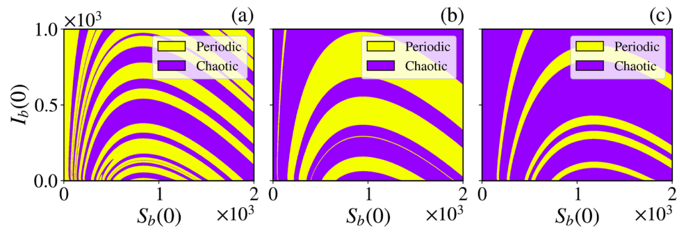
Fig. 5 Basins of attraction in the S_b(0) \times I_b(0) plane for a \chi = 0.32 (region 2), b \chi = 0.36 (region 4), and c \chi = 0.4448 . Yellow and purple denote initial conditions converging to the periodic and chaotic attractors
