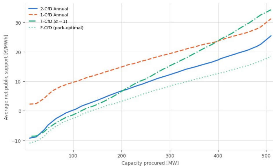
Figure 6. Average net public support against the capacity procured, when projects are awarded contracts in order of cost and each winner receives its own break-even remuneration. Energy-weighted, so the value at each point is the public cost per MWh of the volume procured.
