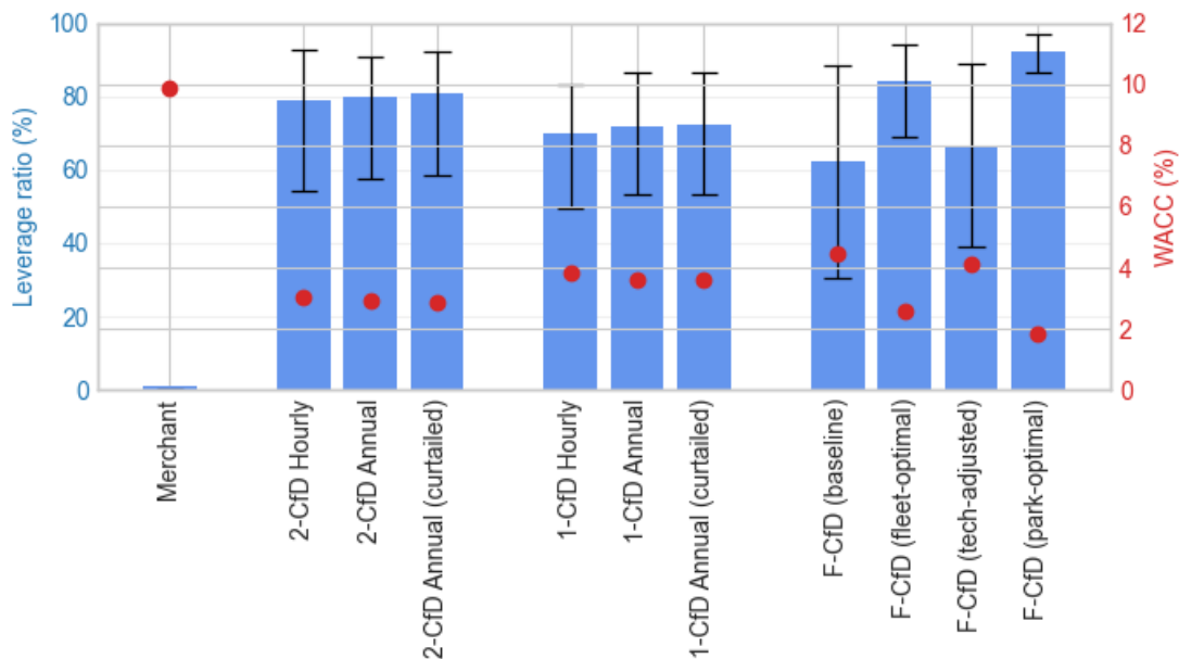
Figure 2. Financial indicators across wind parks under each contract type. Blue bars show the average leverage ratio; whiskers indicate the central 80% (10–90%) of the distribution. Red dots show the average WACC implied by that leverage, based on the assumptions in Table 2.
