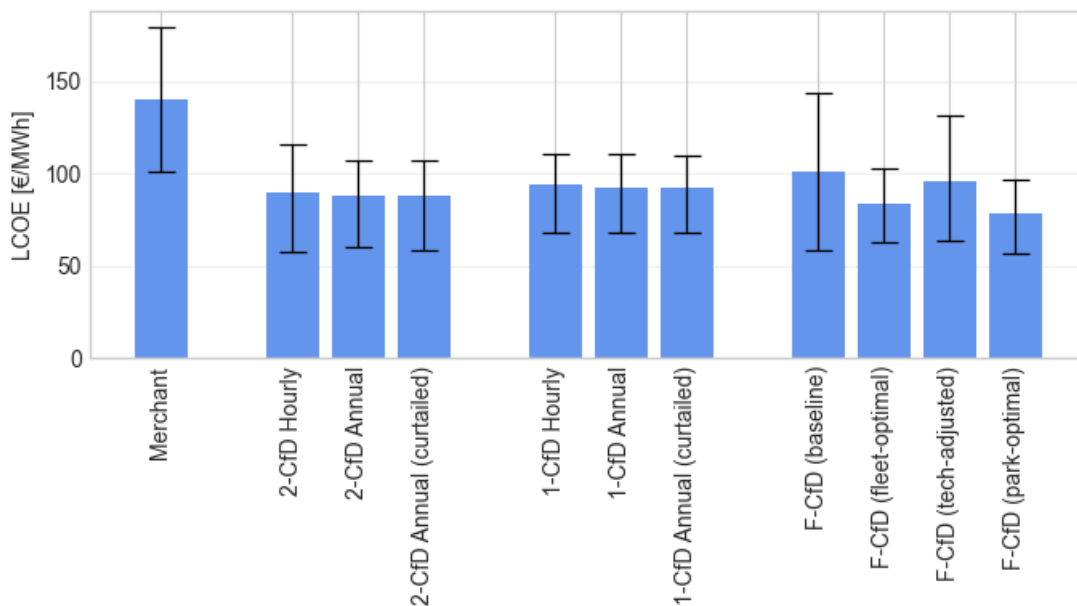
Figure 3. LCOE levels across wind parks under each contract type. Bars show the average LCOE; whiskers indicate the central 80% (10–90%) of the distribution.
