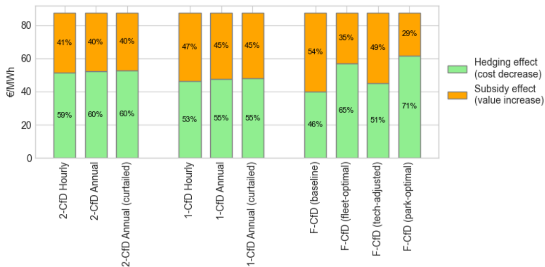
Figure 5. Decomposition of how each contract closes the merchant gap, split into a subsidy effect (a higher average price at which investors sell their electricity) and a risk-reduction effect (a lower LCOE through better financing conditions).
