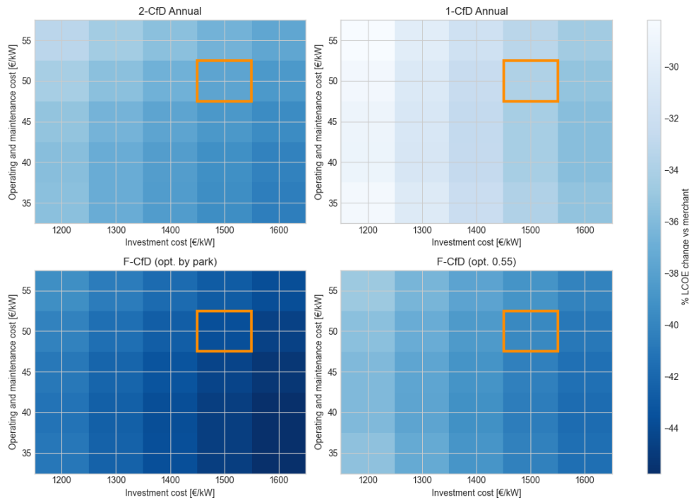
Figure B1. Average reduction in LCOE across wind parks as a function of assumed investment cost and operating-and-maintenance cost. The square highlighted in orange marks the baseline assumptions.
