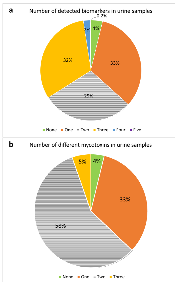
Fig. 1 Number of detected biomarkers and mycotoxins in urine samples of pregnant women in rural Bangladesh ( n = 447 ). Only in 17 urine samples (4%) none of the investigated mycotoxins were detected. About a third of the urine samples contained one, a third two, and another third three detectable mycotoxin biomarkers. Only 2% contained more than three. (Figure 1a). This corresponds to two different mycotoxins detected in over half and three in 5% of the samples, while a third of samples contained one detectable mycotoxin. (Figure 1b). tCIT- total CIT (CIT+ HO-CIT); tDON- total DON (DON + DON-Glucuronides); tAF- total aflatoxins (AFM1+AFB2)
