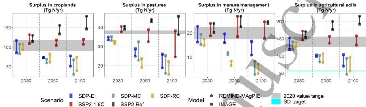
Figure 4: Global nitrogen inputs and surpluses. a Nitrogen (N) inputs on cropland, including inorganic fertilizer, manure, and total N inputs. Total inputs also account for biological fixation and atmospheric deposition. New N fixation denotes the sum of inorganic fertilizer and biological fixation by cultivating leguminous crops. b N surplus in croplands, pastures, and manure management as well as N surplus in agricultural soils, derived as the sum of surplus from croplands and pastures. Indicators are presented for the three SDP scenarios in comparison to a trends-continued reference scenario (SSP2-Ref) and a climate-policy-only scenario (SSP2-1.5C) for the years 2030, 2050 and 2100. Vertical bars depict the model range and symbols indicate results from individual models. The shaded grey bands denote the ranges of modelled values for 2020. The cyan lines display the global boundaries for the respective N indicators (Schulte-Uebbing et al. , 2022). All indicators are described in Suppl. Table S2.
