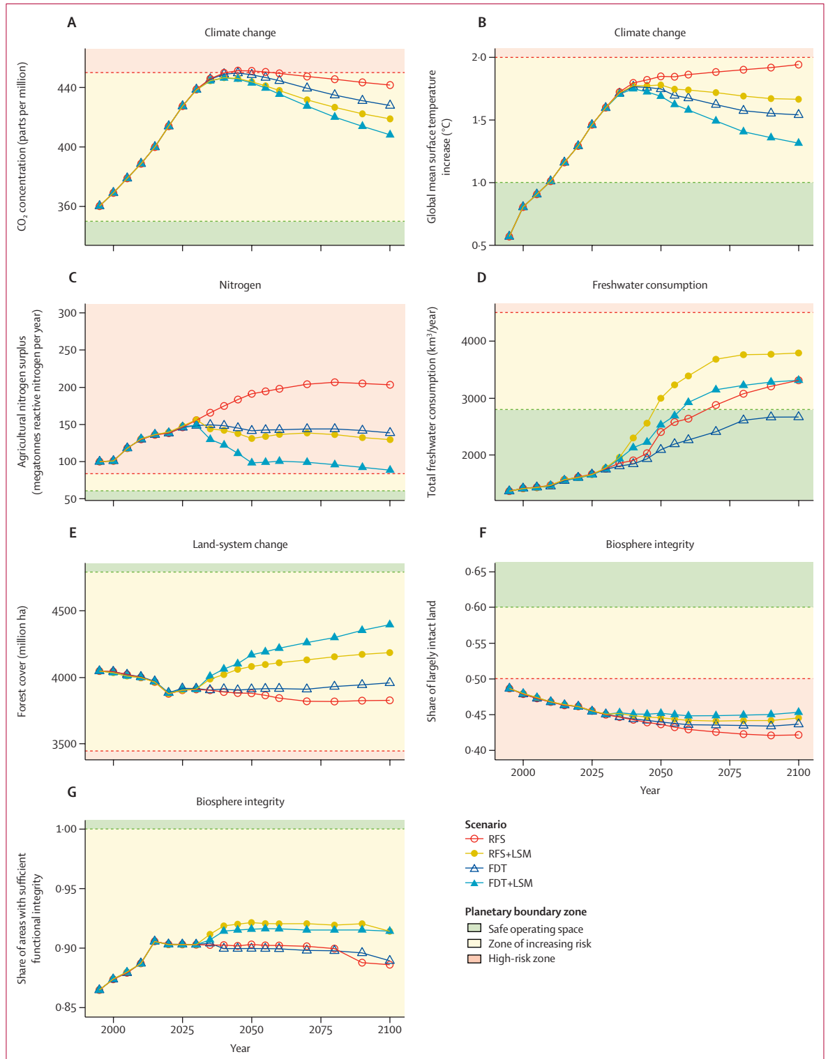
Figure 2: Planetary boundary control variables for the core scenarios over time In all scenarios, ambitious energy-system climate change mitigation is assumed. The green dashed line indicates the safe planetary boundary (ie, the transgression point between the safe operating space and the zone of increasing risk). The red dashed line indicates the transgression point between the zone of increasing risk and the high-risk zone. The upper end of the zone of increasing risk is not defined for the biosphere (functional integrity) planetary boundary (G). FDT=food demand transformation. FDT+LSM=food demand transformation with land-based, supply-side measures. RFS=reference food system. RFS+LSM=reference food system with land-based, supply-side mitigation measures.
