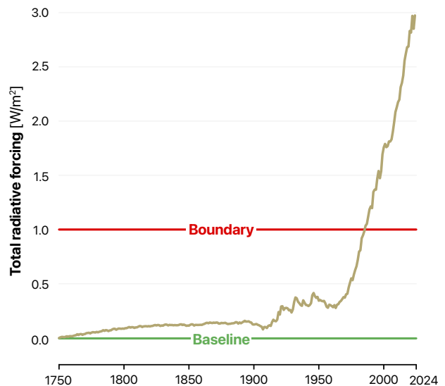
FIGURE 18 - Disturbance of our planet’s energy balance. This figure shows the global average of human-induced radiative forcing at the top of the atmosphere from 1750 to 2024. 242 The values were calculated using observational data and established climate models, based on methods from the IPCC. The green line marks the safe baseline (0.0 W/m 2 ), and the red line indicates the Planetary Boundary (+1.0 W/m 2 ).
