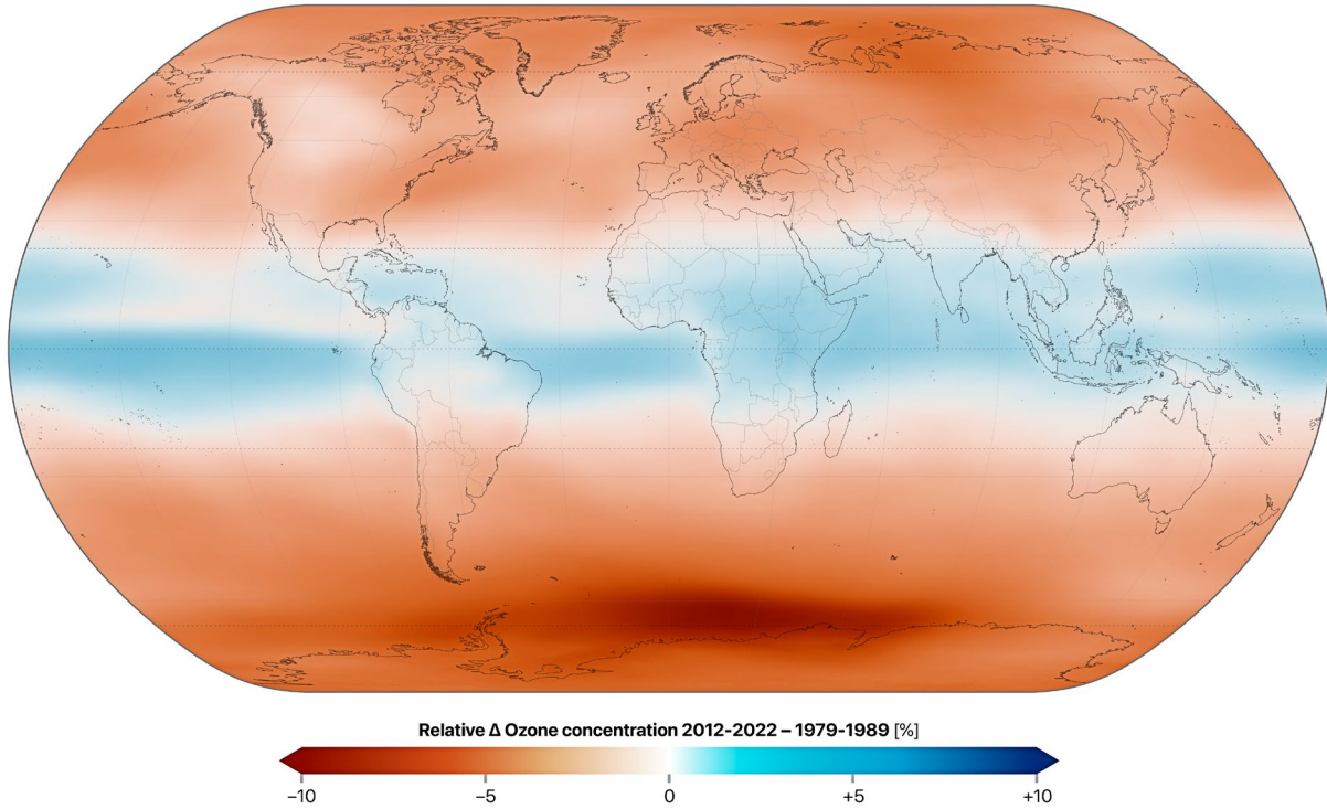
FIGURE 44 - Global map of recent ozone layer changes. This map shows the relative change of the control variable “global mean stratospheric ozone concentration” between 1979-1989 (first 11-year cycle of this data set) and 2012-2022 (last 11-year cycle of this data set, e.g. a change from 260 DU to 273 DU would be indicated by a value of +5 %). Areas where total ozone has increased are shown in shades of blue, and areas where it decreased are shown in shades of red. Data from Copernicus (2020). 373
