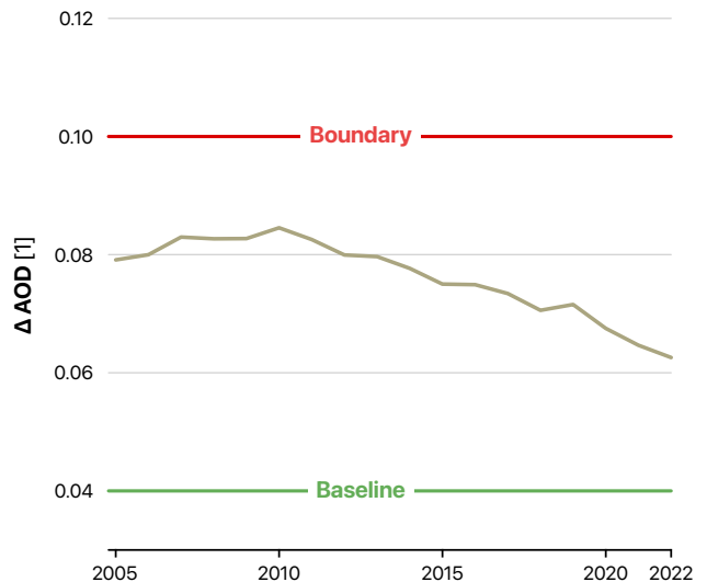
FIGURE 42 - Bridging the divide: Declining interhemispheric difference in Aerosol Loading. This chart shows the 5-year running mean of the difference in the aerosol optical depth (AOD) between the Northern and Southern Hemispheres, calculated by averaging data from 60° north to 60° south for the period from 2003–2024. The red line shows the Planetary Boundary of 0.1, while the green line represents the baseline of 0.04. Data from CAMS EAC4. 360
