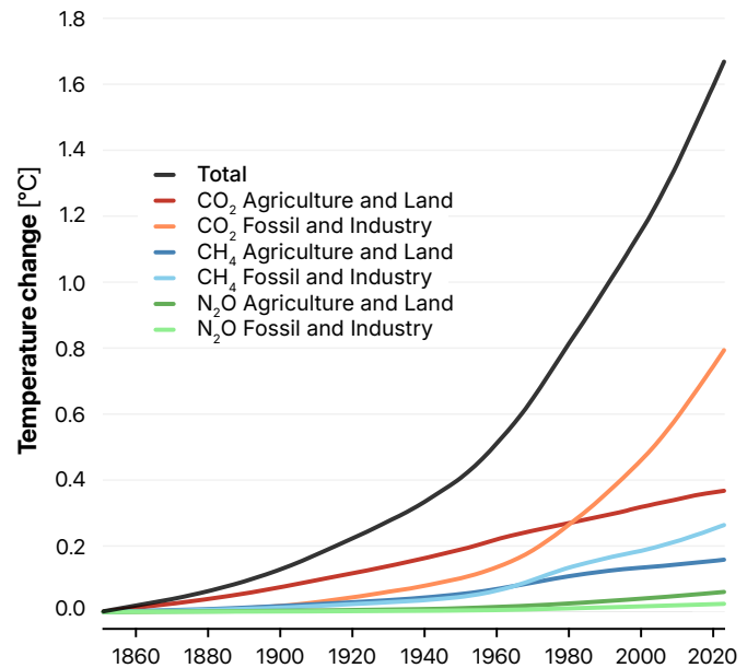
FIGURE 21 - Different gases and sectors contribute unevenly to climate change. The figure shows the temperature contributions from individual greenhouse gases (CO 2 , CH 4 , and N 2 O) over time, with contributions separated by source category (fossil fuels & industry vs. agriculture & land use) 260,261 . These visualizations reinforce the importance of a multi-gas perspective in understanding climate forcing.
